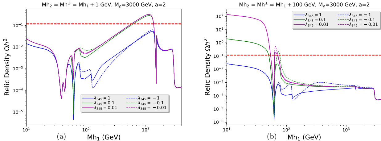
FIG. 3. Relic density \Omega_{\text{DM}} h^2 , as a function of M_{h_1} for different values of \lambda_{345} in a quasi-degenerate scenario (a) where M_{h_2} = M_{h_{\pm}} = M_{h_1} + 1 and a no-degenerate scenario (b) where M_{h_2} = M_{h_{\pm}} = M_{h_1} + 100 . In both cases we fix the values of M_{\rho} = 3000 GeV, a = 2 and \lambda_2 = 1 . The horizontal red line corresponds to the relic density measurements PLANCK limits.
